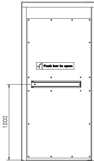
② PUSH SIDE ELEVATION
