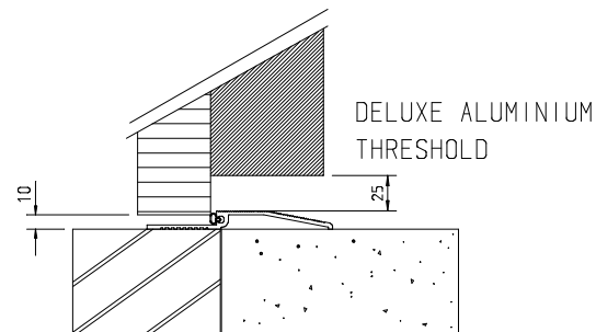
④ THRESHOLD DETAIL
